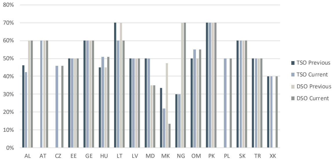
Figure 50 Gearing ratios
