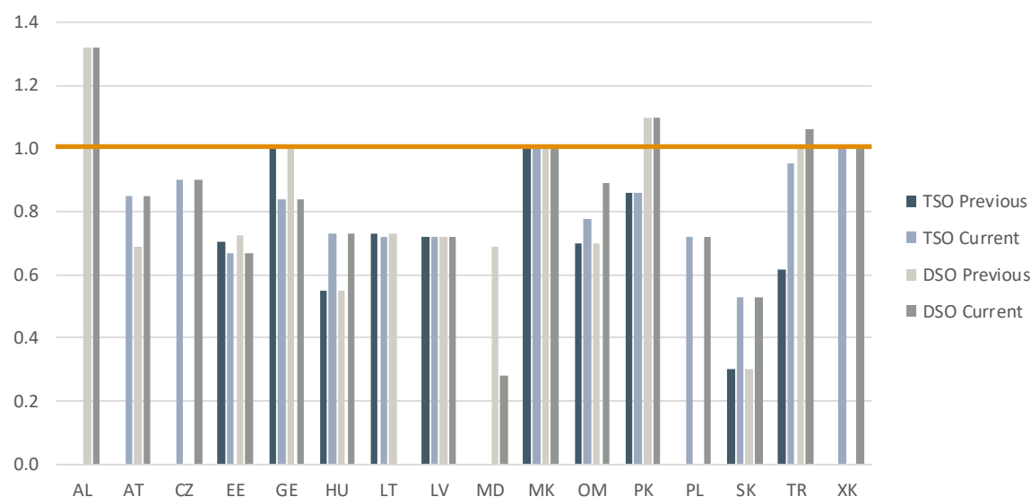
Figure 45 Equity betas
