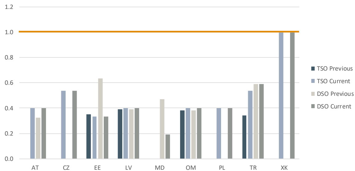
Figure 46 Asset betas
